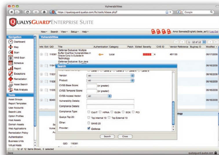
Figure 1: QualysGuard KnowledgeBase with iDefense Exclusives
